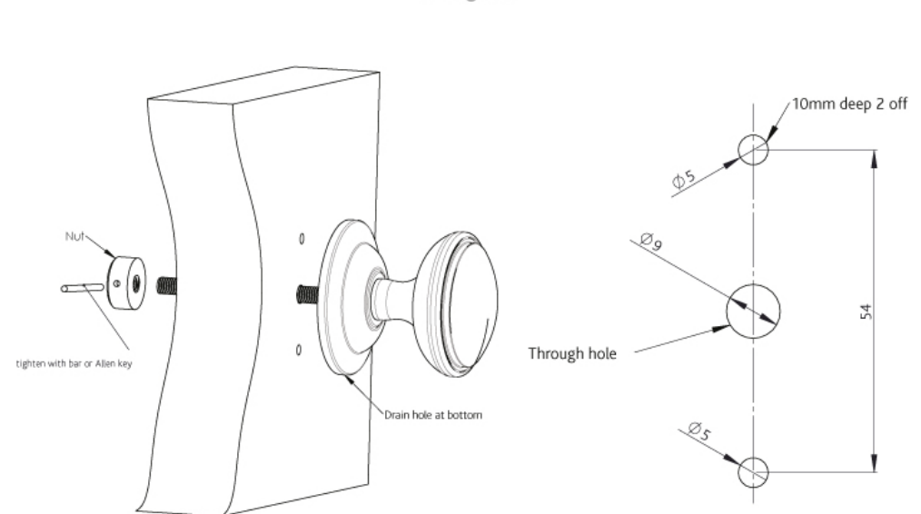
Through Fix
