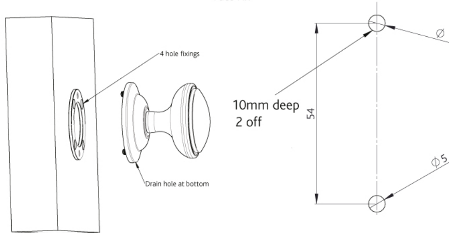
Face Fix
