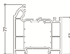
LSC016 48mm Composite Door Outer Frame
